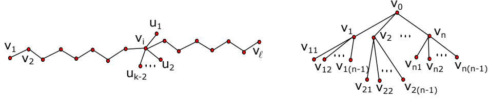
Figure 5: Gadget graphs for addition and squaring.
