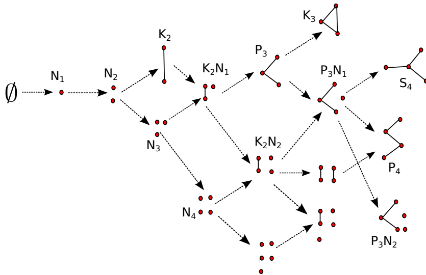
Figure 1: The first few layers of the subgraph order.
