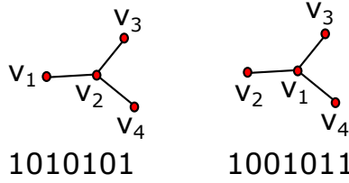
Figure 6: Left: binary representation corresponding to arbitrary labelling of S_4 . Right: uniqueGraph representation of S_4 in binary.
