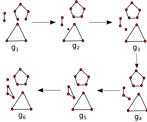
Figure 3: g_1, g_2, g_3, g_4, g_5, g_6 all pac, only g_2, g_5, g_6 soc', only g_5 soc.
